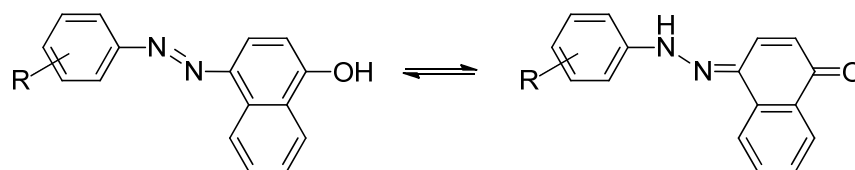
Figure 3: An example of the tautomerism between azo and hydrazone forms (Hunger 2003).
