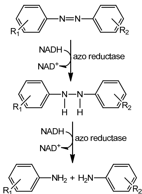
Figure 7: Azoreductase mechanism in the environment (Guo et al. 2010).
