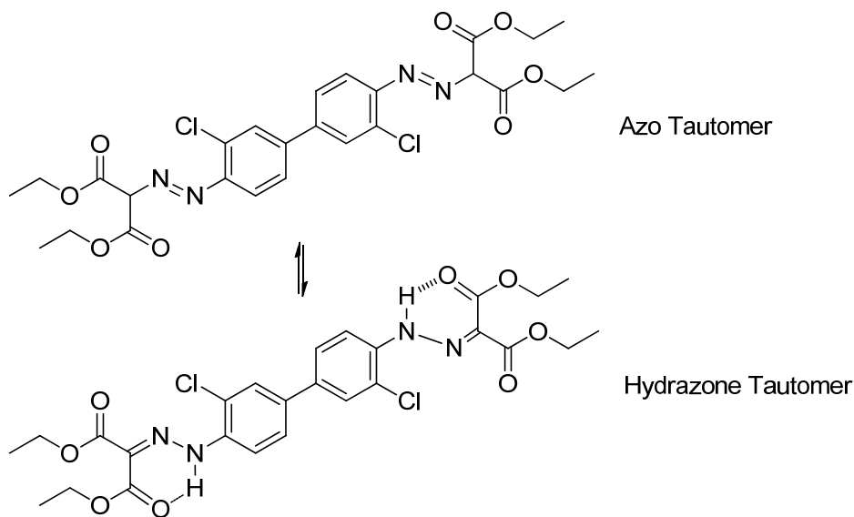
Figure 4: The azo and hydrazone tautomers of a 3,3'-dichlorobenzidine-based colourant disazo coupled to diethyl malonate (De France et al. 1986).
