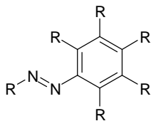
Figure 5: Aromatic azo-based substances.
