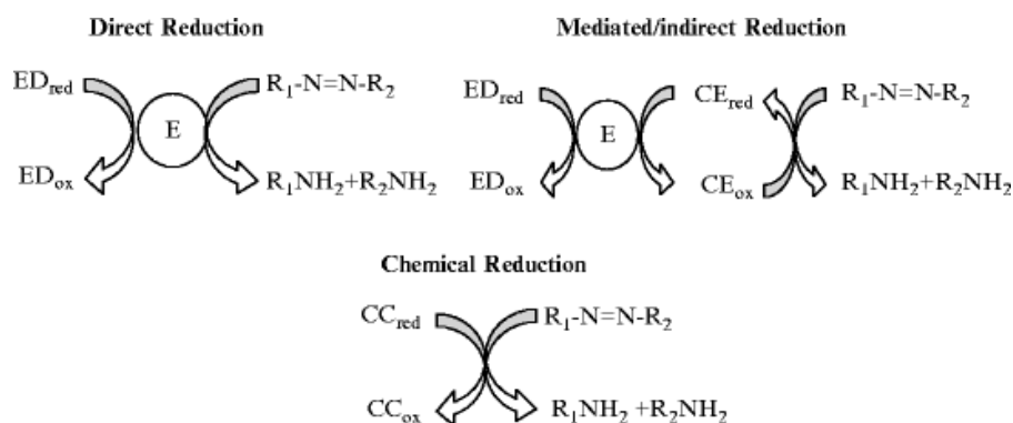
Figure 8: Mechanisms of azo dye bioreduction (Guo et al. 2010).
